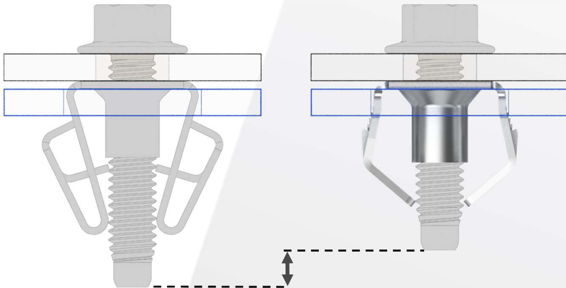
Cost savings due to smaller packaging size and shorter screw compared to existing solutions
